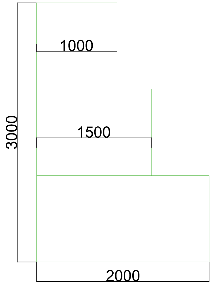
SECTION FOR GABION WORKS 5M U/S & D/S IN BOTH SIDES
