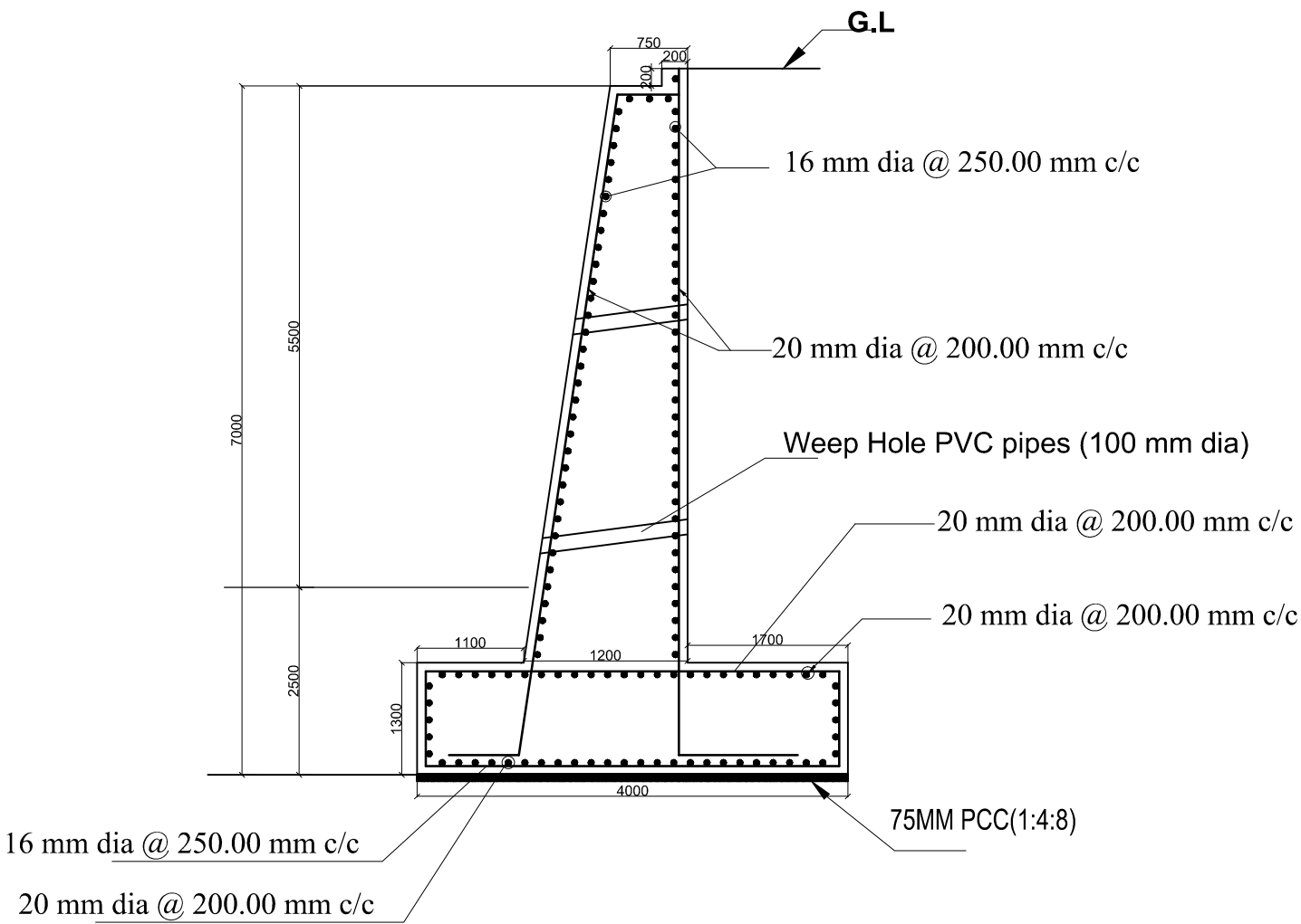
DETAIL OF LEFT AND RIGHT BANK ABUTMENT
