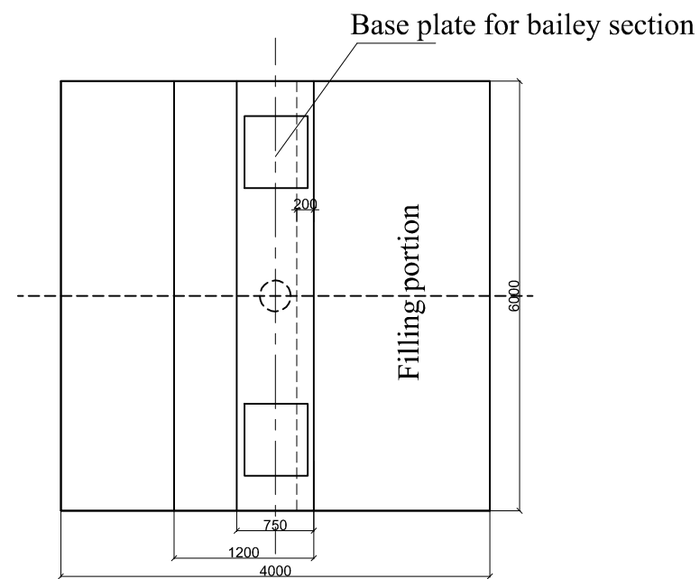
ABUTMENT PLAN
